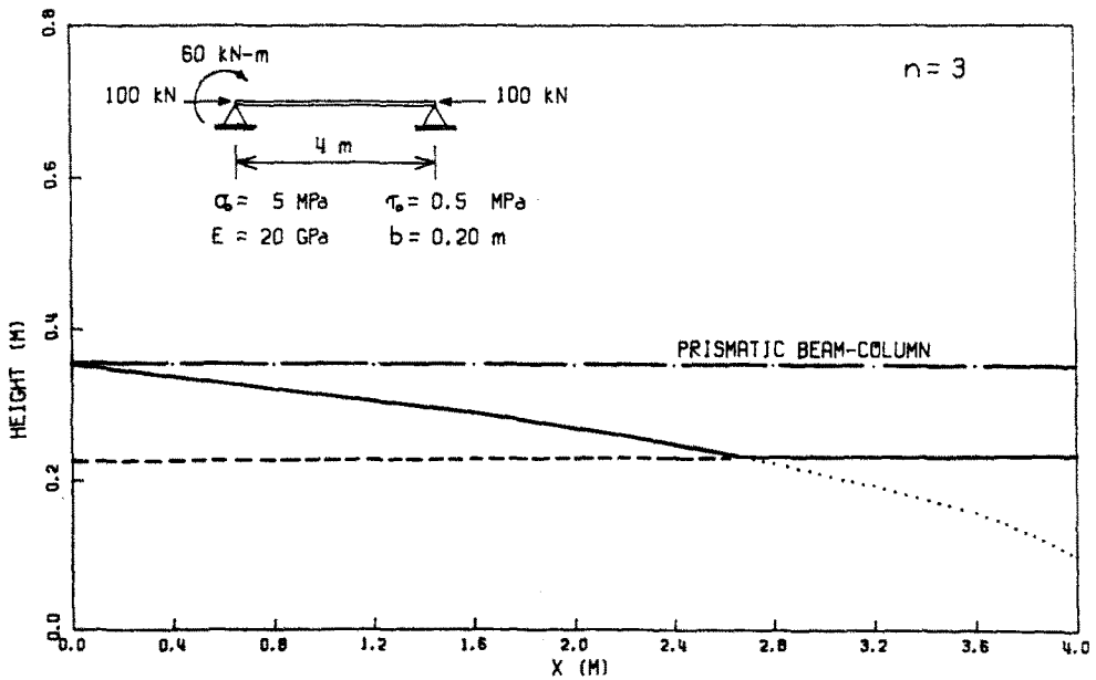
Fig. 11. Optimal design of the structure shown in Fig. 9 for a solid rectangular cross-section of constant width and variable depth, n = 3 .
